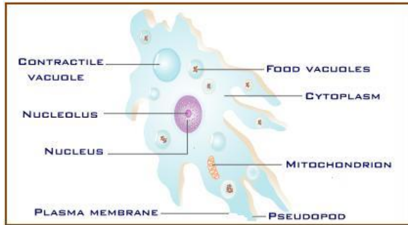
Amoeba
